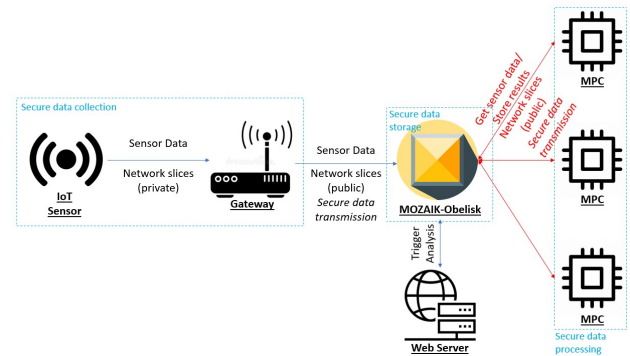
Figure 1: MOZAIK architecture overview
